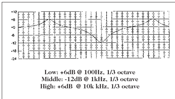
Graphic Equalizers
