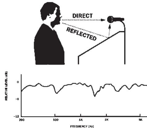
Reflection Pickup
