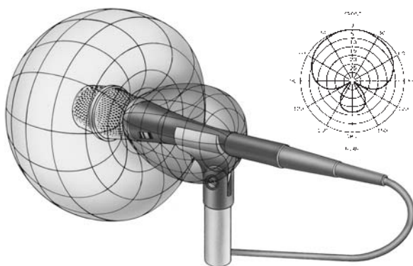
Supercardioid Microphone
