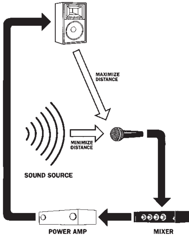
Acoustical and Electrical Feedback Path
