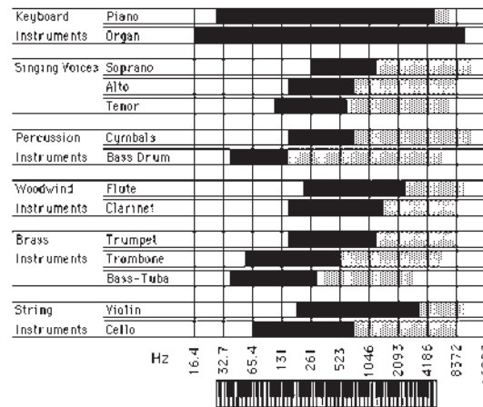
Instrument Frequency Ranges
