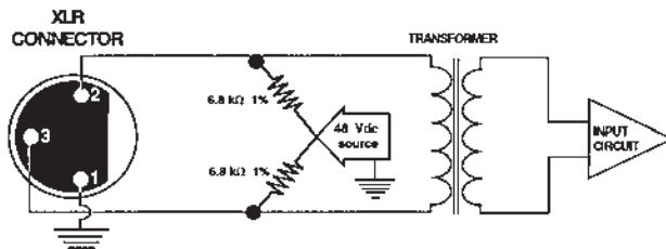
Phantom Power Schematic
